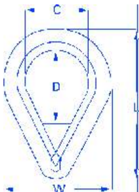
Pennant Thimbles
