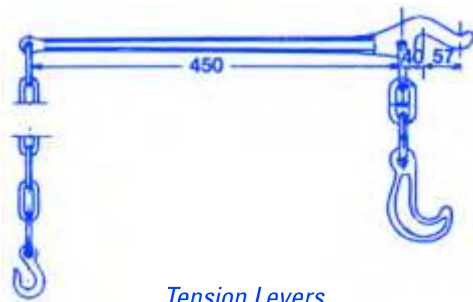
Tension Levers
