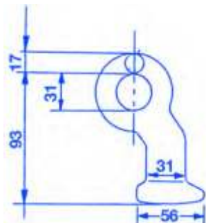
Elephants Feet
