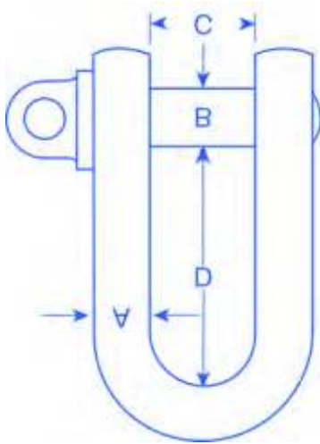
Dee Shackles
