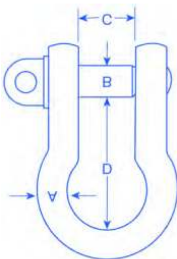
Commercial Bow Shackles
