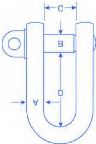
Commercial Dee Shackles
