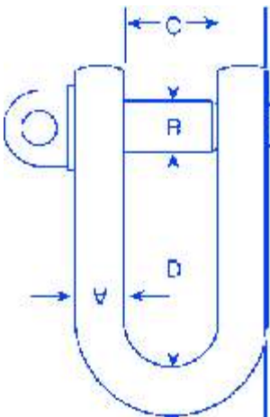
Screw Pin Dee Shackle
