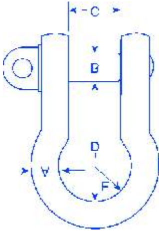
Screw Pin Bow Shackle
